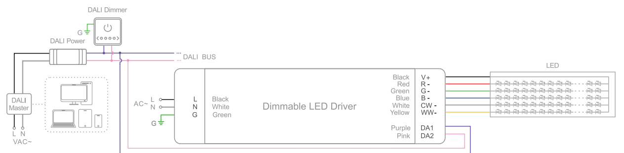
Diagram 5 DALI Master
